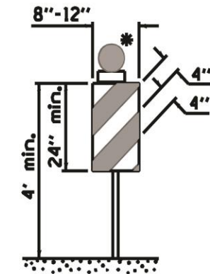
VERTICAL PANEL POST MOUNTED
