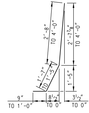
#6d (E) BAR
