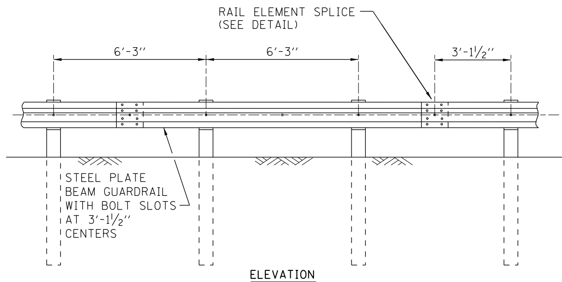
TYPE A 6'-3" TYPICAL POST SPACING
