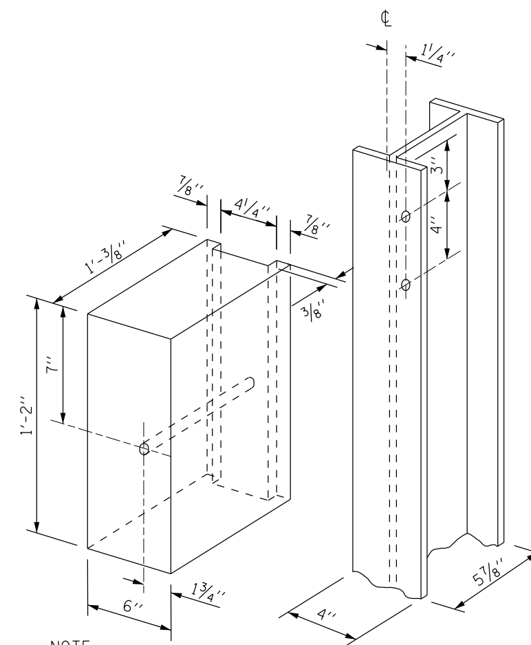
WOOD BLOCK-OUT AND STEEL POST DETAILS
