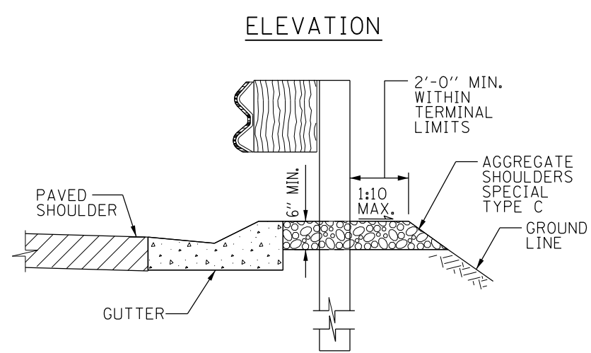
WITH TYPE G-2 GUTTER SECTION A-A
