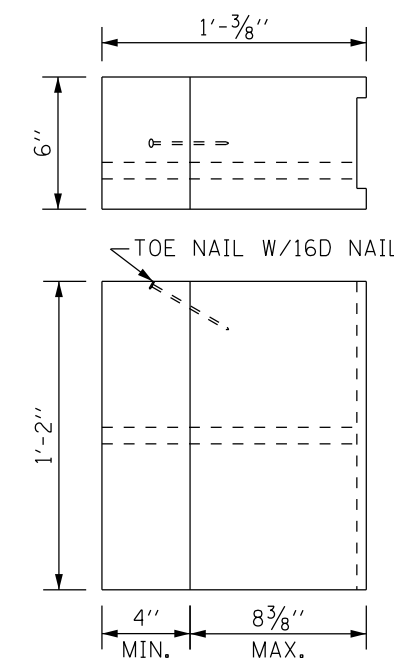
TWO-PIECE WOOD BLOCKOUT OPTION
