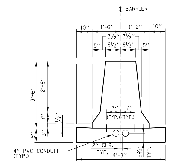
CONCRETE BARRIER, DOUBLE FACE, 42" CONCRETE BARRIER BASE SECTION A-A
