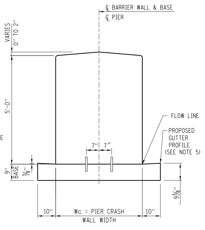
SECTION C-C
