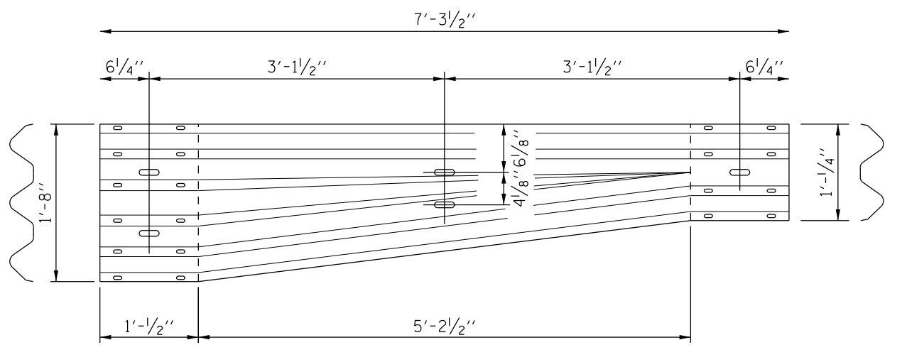
TRANSITION SECTION
