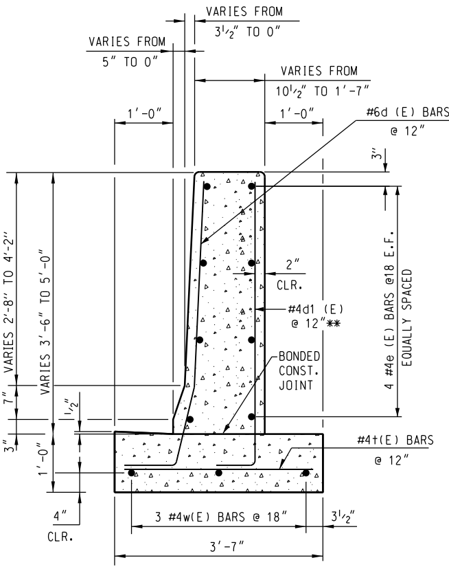
SECTION B-B
