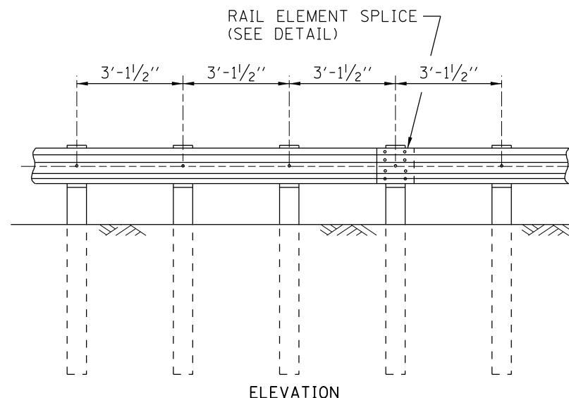
TYPE B 3'-1/2" 1/2 POST SPACING
