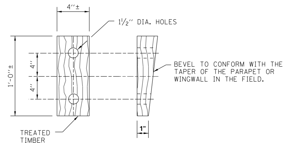
WEDGE M
