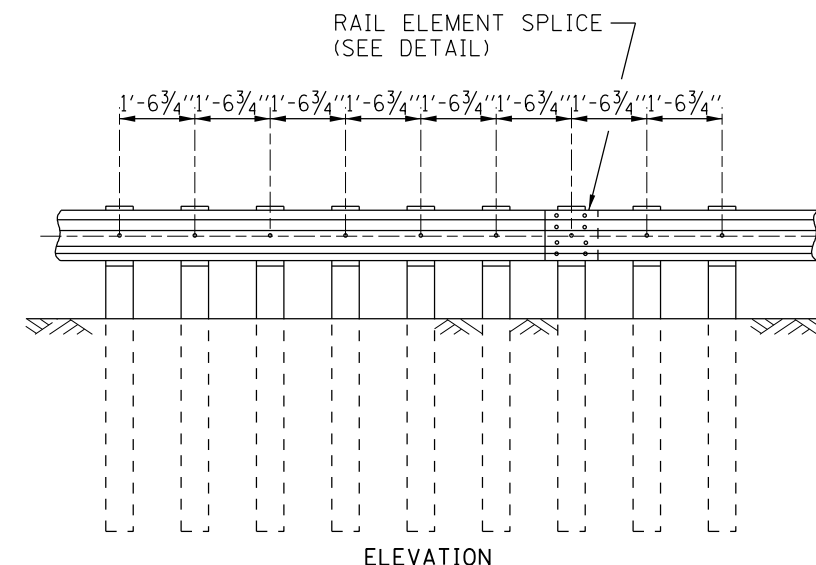
TYPE C 1'-6 3/4" 1/4 POST SPACING
