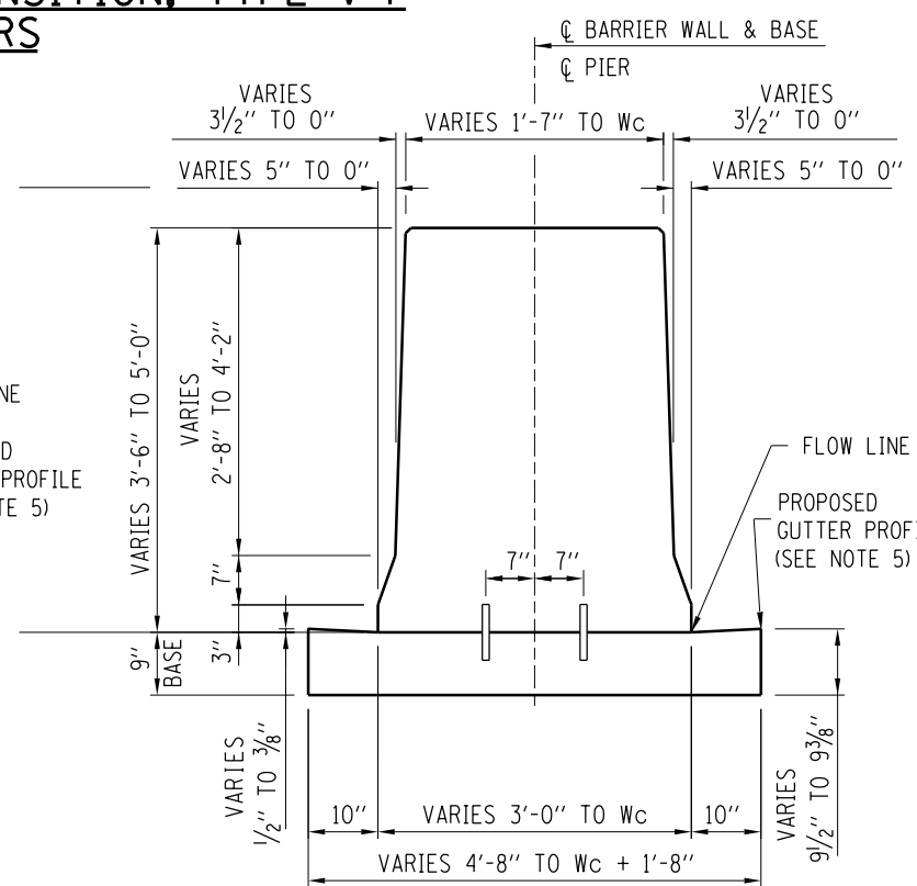
SECTION B-B
