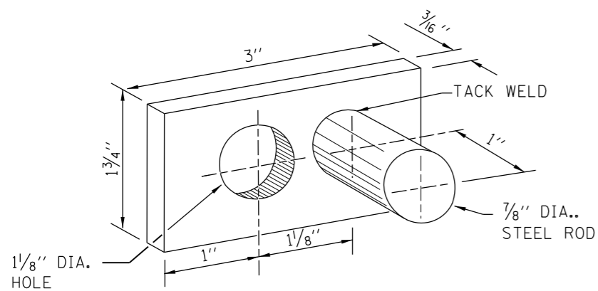
PLATE WASHER D
