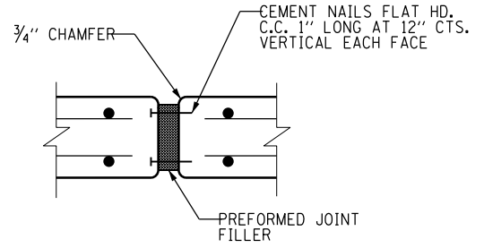
EXPANSION JOINT
