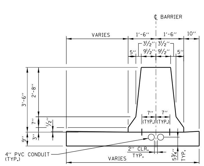
CONCRETE BARRIER, DOUBLE FACE, 42" CONCRETE BARRIER BASE SECTION B-B
