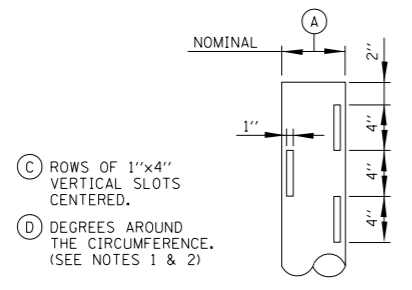
DETAIL A - SLOTTED INLET
