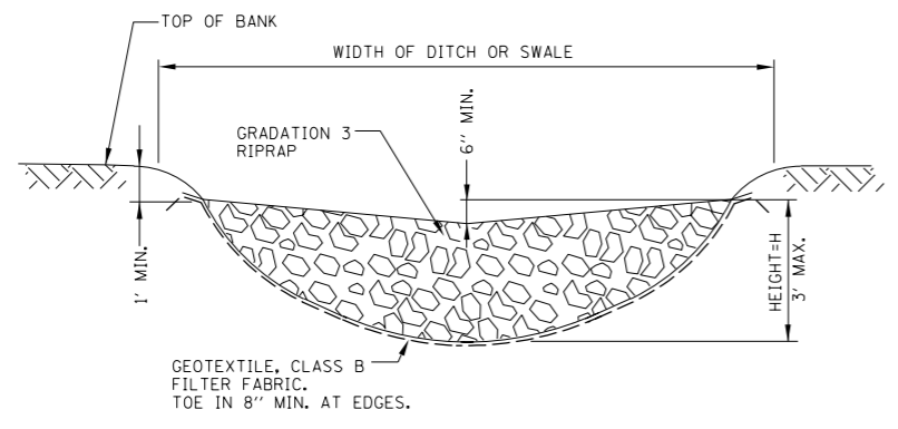
CROSS SECTION CENTERLINE LOOKING DOWNSTREAM
