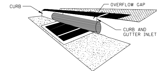
INLET DAM
