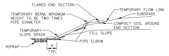
SECTION A-A FOR FILL SLOPES
