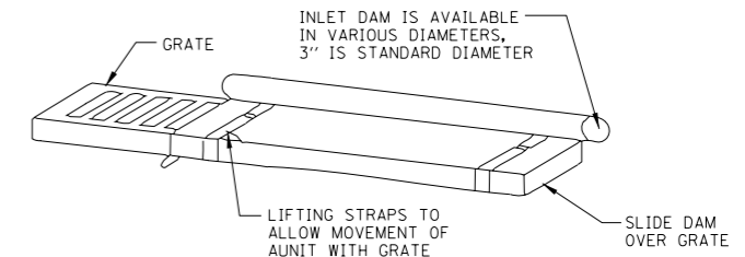
INLET BASKET (SEE NOTE 3 BELOW)
