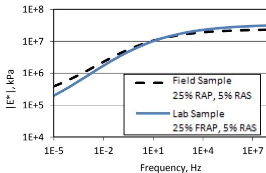
Figure 4-27. Base course field vs. lab
