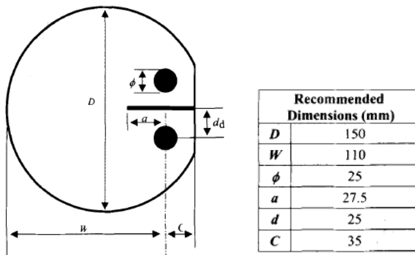
Figure 3-13. Completed DC(T) Specimen and ASTM-specified Dimensions
