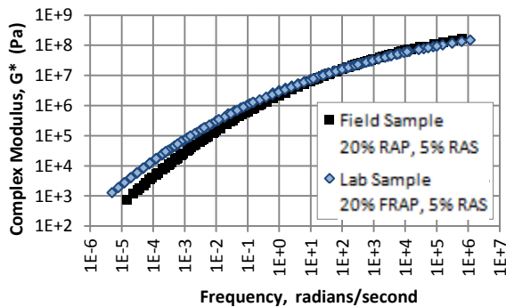
Figure 4-14. Surface course field vs. lab
