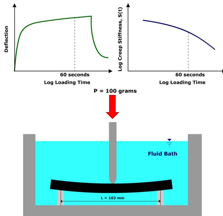
Figure 3-8. Bending beam rheometer test (www.pavementinteractive.org)
