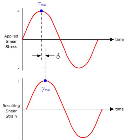
Figure 3-6. Relationship between phase angle and time (www.pavement interactive.org)
