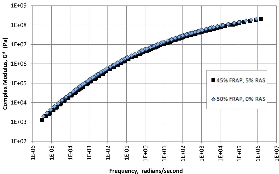
Figure 4-7. Master curves of binder from base course mixes with 50% recycled materials
