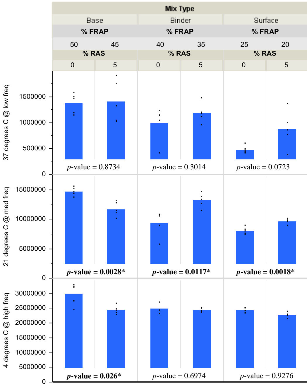
Figure 4-23. t-test results comparing E* values of mixes with RAS and no RAS
