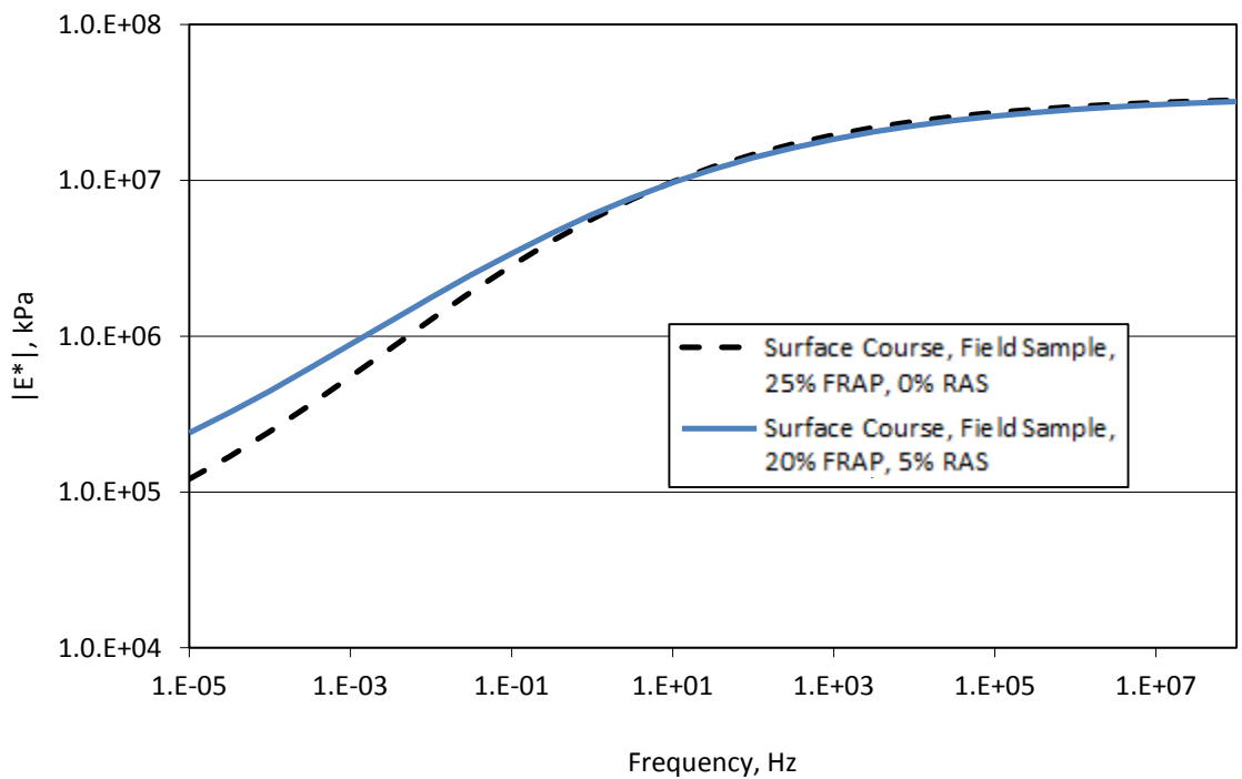
Figure 4-22. E* Master curves for surface course field samples
