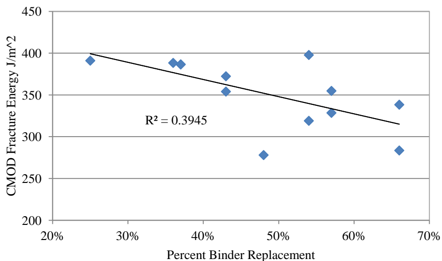
Figure 4-40. Fracture energy vs. percent binder replacement
