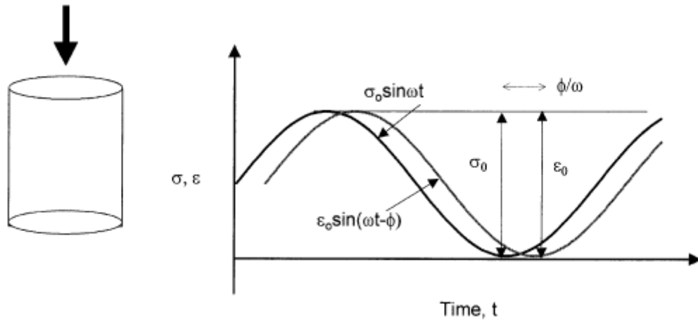
Figure 3-11. Haversine loading for the dynamic modulus test (NCHRP Report 547)
