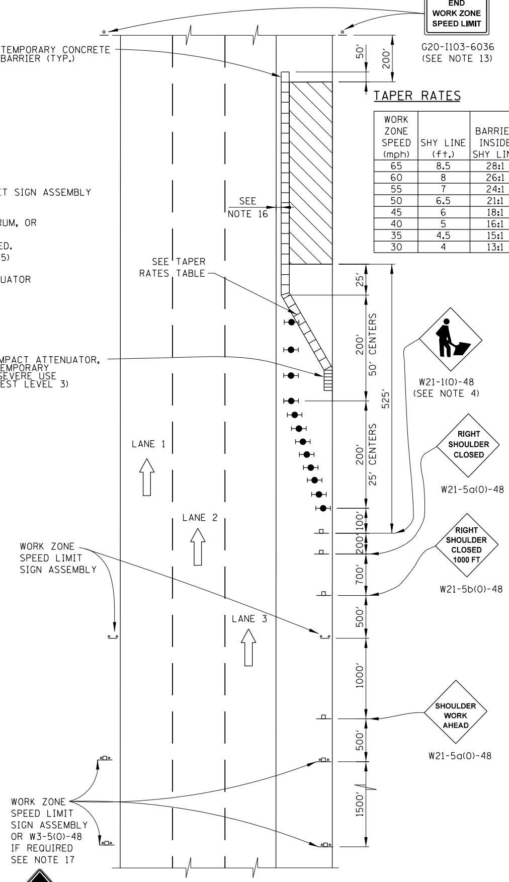
WORK ZONE WITH BARRIERS N.T.S.
