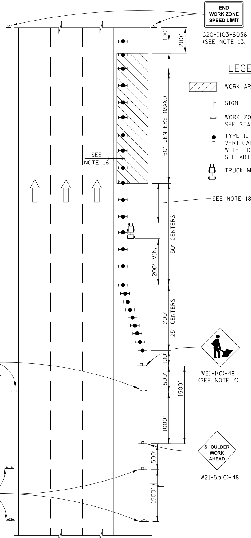
WORK ZONE WITH BARRICADES N.T.S.
